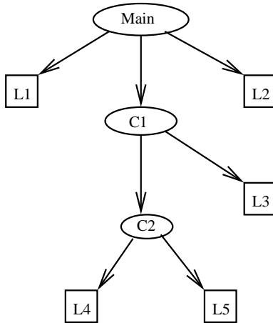
Figure 2 The Rec-I-DCM3 decomposition: main problem, composite subproblems (C1-C2) and leaf subproblems (L1-L5).
